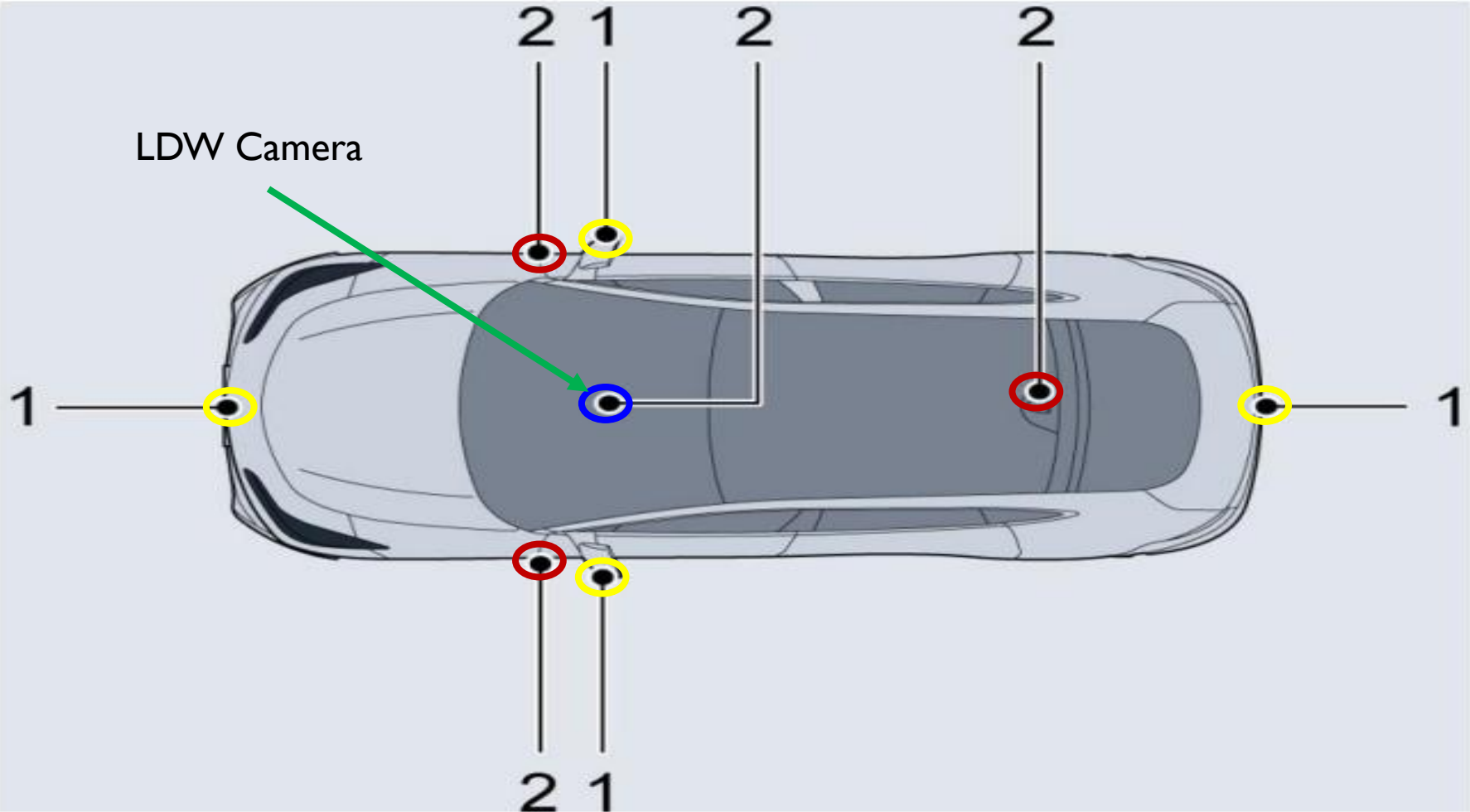
Installation Position of Cameras
