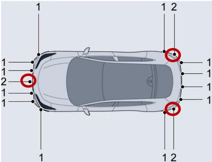
Installation Position of Radars
